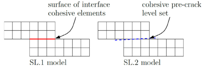
Fig. 5. Visualization of the two different single lap models.
