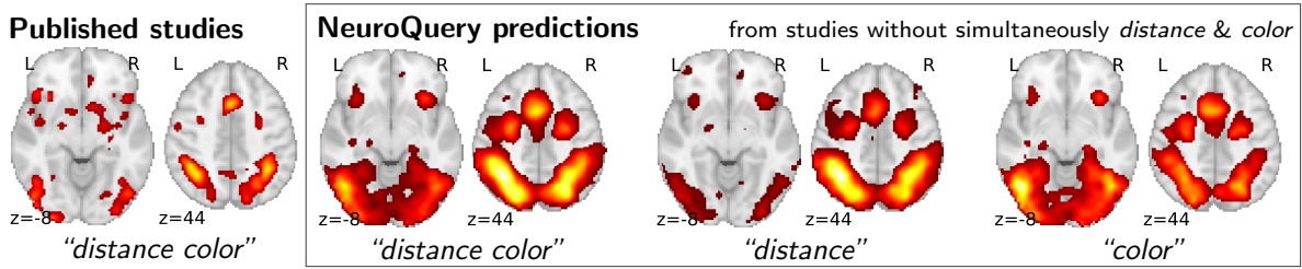
Figure 3: Mapping an unseen combination of terms Left The difference in the spatial distribution of findings reported in studies that contains both “distance” and “color” ( n = 687 ), and the rest of the studies. – Right Predictions of a NeuroQuery model fitted on the studies that do not contain simultaneously both terms “distance” and “color”.
