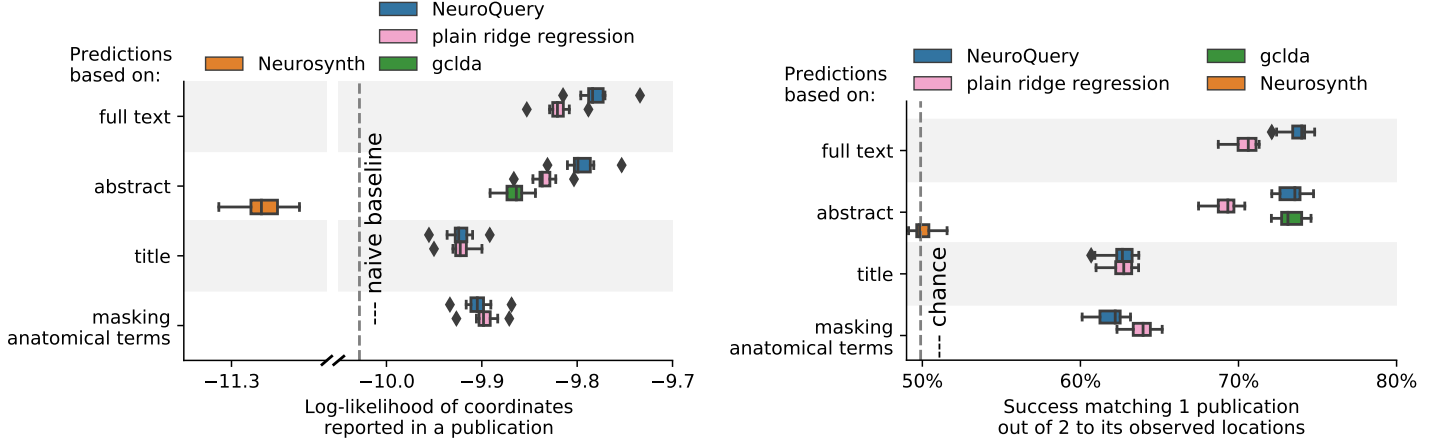
Figure 11: Explaining coordinates reported in unseen studies. left: log-likelihood of reported coordinates in test articles. right: how often the predicted map is closer to the true coordinates than to the coordinates for another article in the test set [Mitchell et al., 2008]. The boxes represent the first, second and third quartiles of scores across 16 cross-validation folds. Whiskers represent the rest of the distribution, except for outliers, defined as points beyond 1.5 times the IQR past the low and high quartiles, and represented with diamond fliers.
