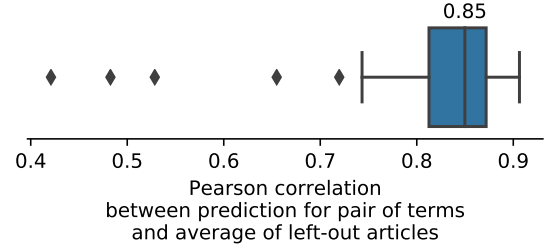
Figure 10: Consistency between prediction of unseen pairs and meta-analysis The Pearson correlation between the map predicted by NeuroQuery on a pair of unseen terms and the average density of locations reported on the studies containing this pair of terms (hence excluded from the training set of NeuroQuery).
