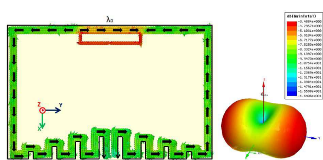
Figure 14. Current distribution and radiation pattern of the full-wavelength dipole on HFSS.
