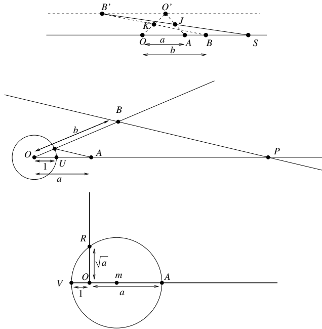
Fig. 3 Constructions for the arithmetic operations. On the top of the figure, sum of a = \overline{OA} and b = \overline{OB} , point O' is any point not on the x axis, K is the midpoint of OO' , and J is the midpoint of O'A ; in the middle, product of a = OA and b = OB , O has coordinates (0, 0) , U has coordinates (1, 0) and OP = ab (note that divisions can be constructed in the same way); at the bottom, square root of a = OA , V has coordinates (-1, 0) , the circle has diameter VA and \sqrt{a} = OR .
