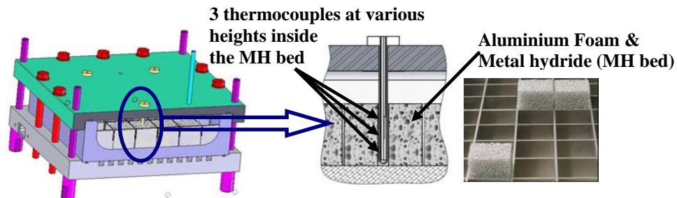
Fig 2- Repartition of the three thermocouples at different levels inside the MH bed.
