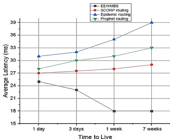
Figure 4. Delivery Probability
