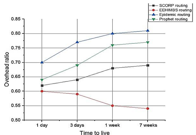
Figure 5. Overhead Ratio
