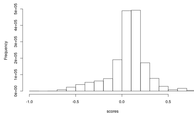
Figure 1: Distribution of token silhouette scores
