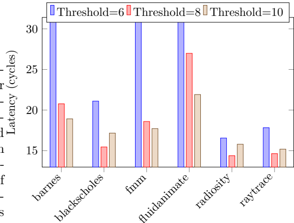
Figure 4: Latency under different threshold values for applications belonging to PARSEC and SPLASH2 benchmark suit.
