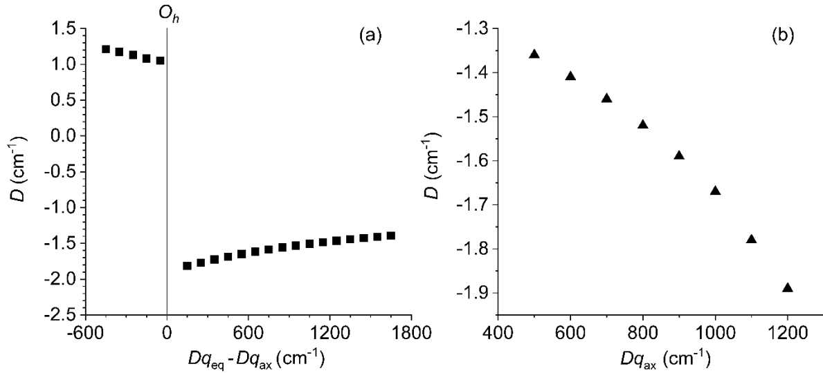
Figure 3. Calculated D value for a 3d^4 ML_4X_2 system in D_{4h} symmetry: (a) as a function of the difference between equatorial and axial LF strength [ (e_{\pi c} + e_{\pi s})/e_{\sigma} = 0.3 for all ligands]; (b) as a function of axial
