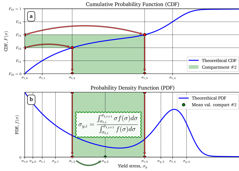
Figure 4: The Distribution Discretization Procedure (DDP): (a) The CDF is split vertically into N equal parts separated by N+1 threshold values F_{t,i} . The CDF is inversed reversed and stress threshold values \sigma_{t,i} are determined. (b) The yield stress values \sigma_{y,i} are calculated as the average value of the distribution's PDF f over the [\sigma_{t,i}, \sigma_{t,i+1}] interval.
