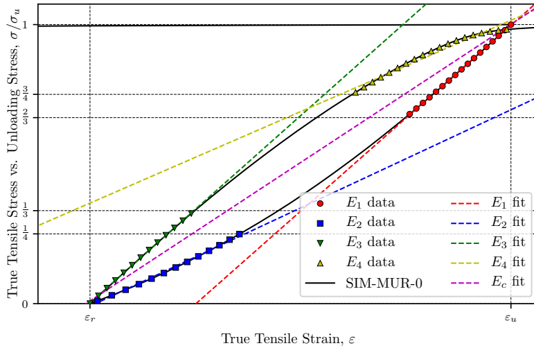
Figure 10: Schematical representation of the procedure introduced by Chen et al (2016b) in order to calculate the 5 moduli E_1 , E_2 , E_3 , E_4 and E_c for each unloading reloading cycle. The vertical axis represents the normalized true stress \sigma/\sigma_u , where \sigma_u is the true stress at the beginning of the unloading step. Each modulus is defined as the slope of a linear fit obtained over a given subset of the data points depending on which modulus is calculated.
