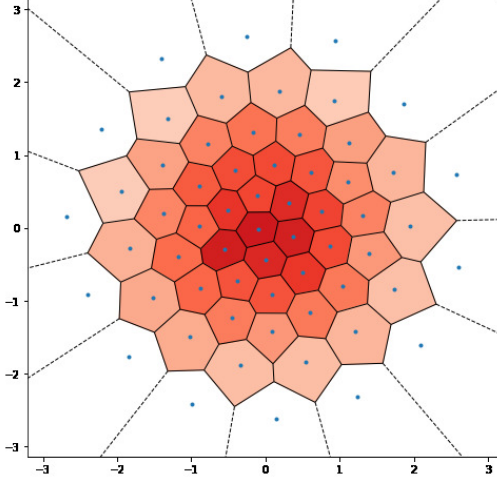
Figure 1: An optimal quantizer for \mathcal{N}(0, \mathbf{I}_2) at level 60.
