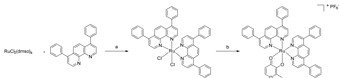
Scheme 1. Synthesis of [Ru(DIP) 2 (mal)](PF 6 ). a) LiCl, DMF, reflux, 24 h, 78%; b) (i) NaOH, maltol, ethanol, reflux, 3 h; (ii) NH 4 PF 6 , ethanol/H 2 O (1:10), yield: 90%.
