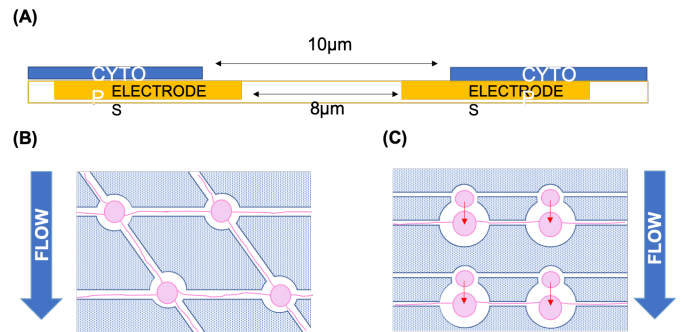
Figure 3: Concept of trap and drop device using dielectrophoresis technique. (A) primary neurons are attracted to the ITO glass coated with CYTOP patterned layer when electric field is applied. (B) primary neurons are dropped into a bigger well made with PDMS allowing (C) cells to grow.
