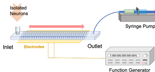
Figure 2: Overview of the trap and drop system
