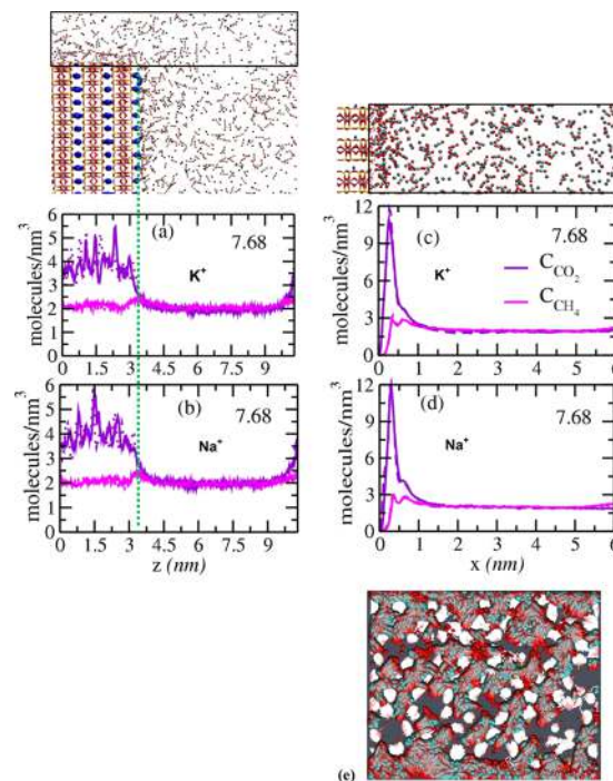
Figure 7. Computed PDPs of CCO 2 (violet) and CCH 4 (magenta) near the broken and protonated (010) surfaces with K + and Na + . The left column represents the average concentrations within 1.50 nm of the surfaces plotted parallel to them for the pore thicknesses shown at the top of the box. (a) K + and (b) Na + . Solid and dashed lines represent the distributions on the left and right sides of the illite models. Green dotted lines in (a) and (b) represent the plane of basal oxygen atoms of the (010) surface. The right column shows the distributions normal to the (010) surfaces. (c) K + and (d) Na + . (e) The adsorption environments of CO 2 molecules in the shoulder region near the protonated (010) surface (0.0–0.2) nm from the surface, comparable to Figure 6. Red and white sticks represent the protonated edges of the (010) surfaces. CO 2 molecules are represented in red (O) and cyan (C).
