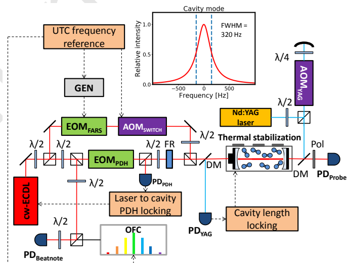
Fig. 1. The frequency-stabilized cavity ring-down spectrometer FS-CRDS referenced to the primary frequency standard UTC (AOS). Light from a continuous-wave external cavity diode laser (cw-ECDL) is polarization split into two beams. One of them is used for PDH locking of the ECDL frequency to the cavity mode and to determine its absolute frequency by measuring the heterodyne beat with the OFC. EOM_{PDH} modulates the phase of light to create the PDH error signal. Second beam probes the gas sample inside the cavity by ring-down decay signals initiated by an acousto-optic modulator ( AOM_{SWITCH} ). The cavity length is actively stabilized to the iodine stabilized Nd:YAG laser. The EOM_{FARS} , also referenced to the UTC (AOS), is used for fast full-spectrum scanning by stepping a laser sideband to successive optical cavity modes. FR – Faraday rotator, GEN – generator, DM – dichroic mirror, Pol – polarizer, and PD – photodiodes.
