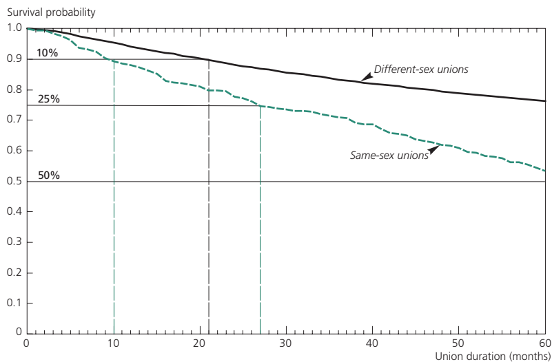
Figure 1. Union survival probability by gender composition
