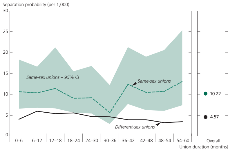
Figure 2. Separation probabilities by duration and gender composition of unions
