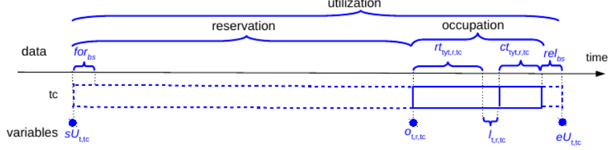
Figure 1: Main variables and data concerning the utilization of tc belonging to route r of train t .
