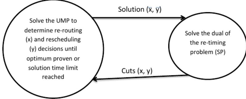
Figure 2: Representation of the classic Benders approach applied to the RECIFE-MILP formulation.
