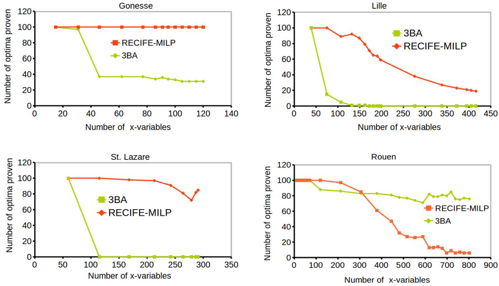
Figure 10: Comparison of the number of instances solved to the optimum by RECIFE-MILP and 3BA on the four control areas depending the number of x -variables.
