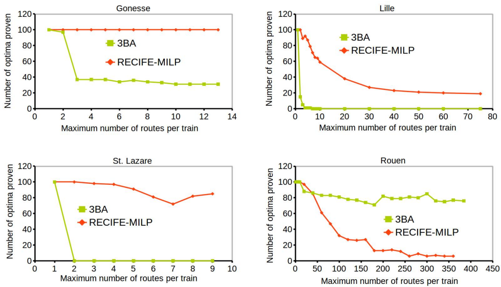
Figure 9: Comparison of the number of instances solved to the optimum by RECIFE-MILP and 3BA on the four control areas depending the maximum number of routes per train.
