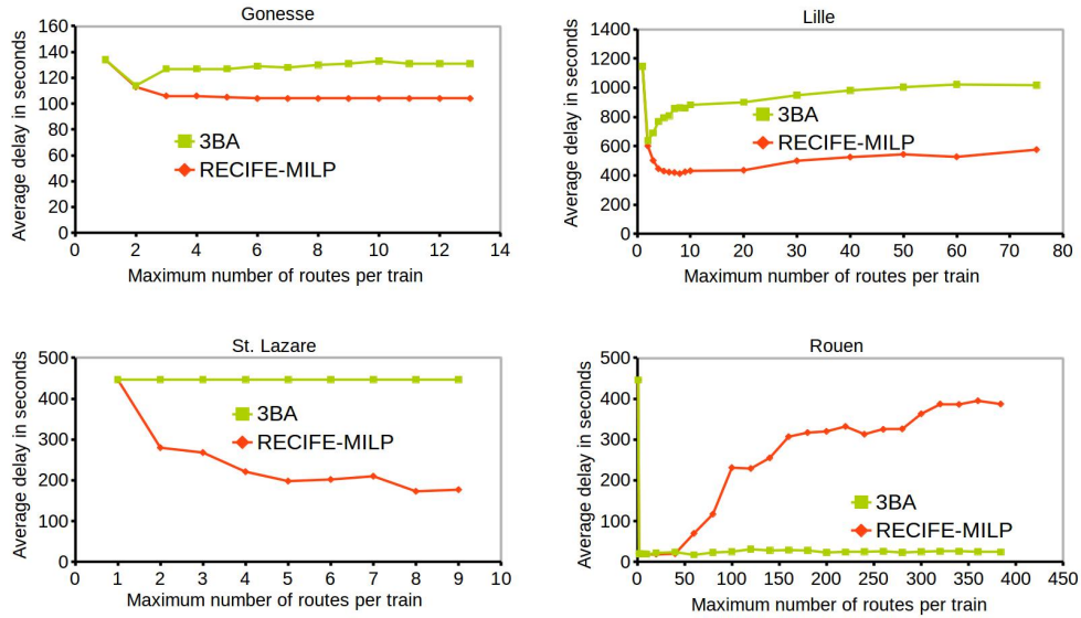
Figure 8: Comparison of the average delay achieved by RECIFE-MILP and 3BA on the four control areas depending the maximum number of routes per train.
