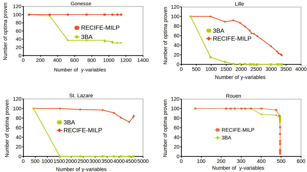
Figure 11: Comparison of the number of instances solved to the optimum by RECIFE-MILP and 3BA on the four control areas depending the number of y -variables.
