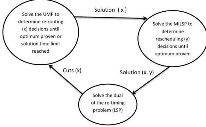
Figure 3: Representation of the three-step Benders Algorithm applied to the RECIFE-MILP formulation.
