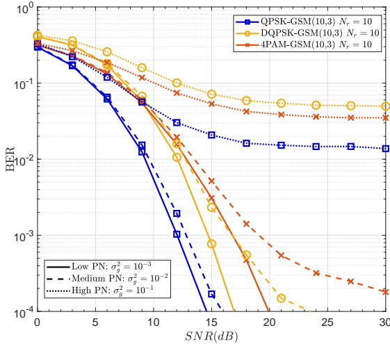
Fig. 3: BER performance of different APM-GSM systems with sub-THz impairments. The spectral efficiency is 12bpsu and both systems are subjected to phase noise with different levels using DO setup. The concerned sub-THz indoor MIMO channels are generated using URA array geometry with 4\lambda antenna separation and N_r = 10 . The AP-MS distance is d = [2m, 8m] with d_{mean} = 5m .
