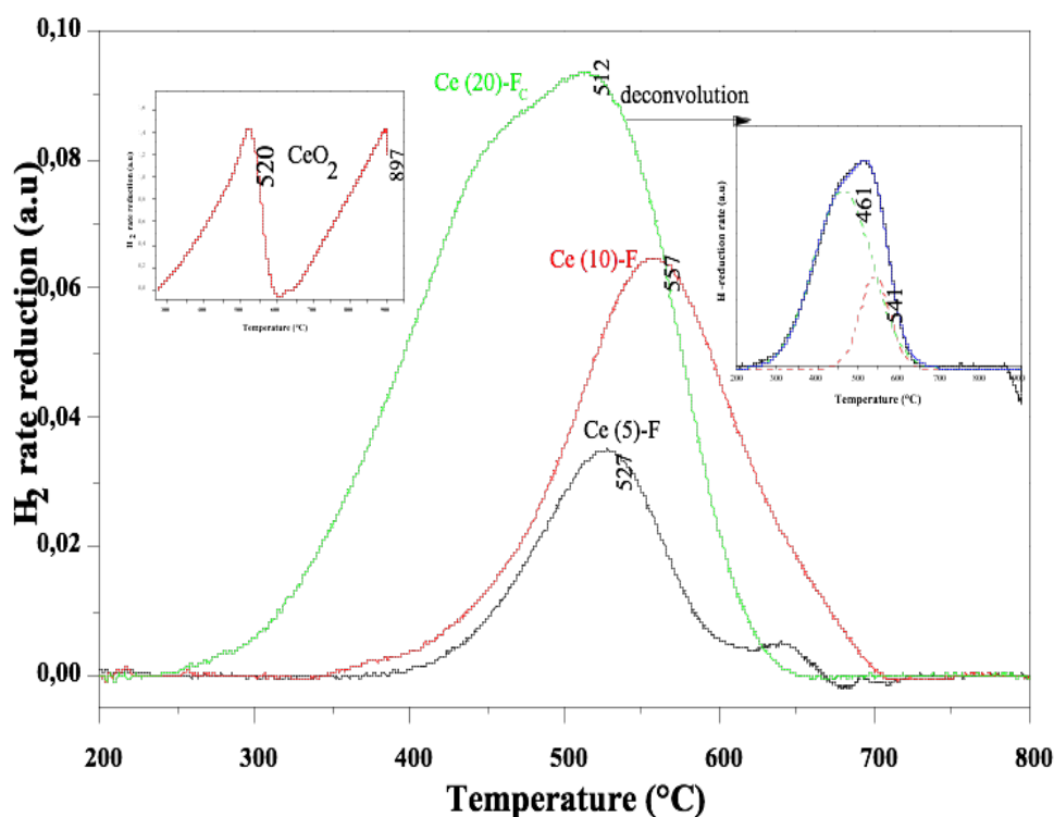
Figure 8 : H_2 -TPR of Ce(5)-F , Ce(10)-F and Ce(20)-F_C and pure CeO_2 .
