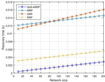
Fig. 12. Recovery time for the different Redundancy Protocols
