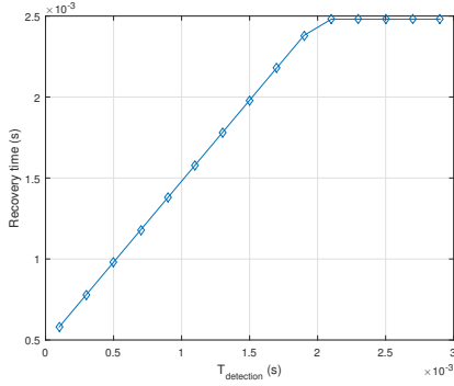
Fig. 8. The impact of T_{detection} on the Maximum Recovery Time for ( M = 40 , T_{detection} \in [0.1 : 0.2 : 3]ms )
