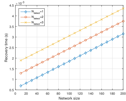
Fig. 10. The impact of N_{detect} on the Maximum Recovery Time vs the Network Size for ( M \in [10 : 10 : 200] , N_{detect} \in [1 : 1 : 3] , P_{local\_detect} = \text{high} )
