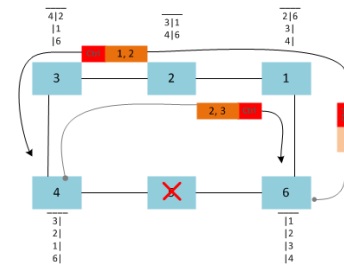
Fig. 5. The QoS-ARRP Auto-configuration Mechanism after a failure detection
