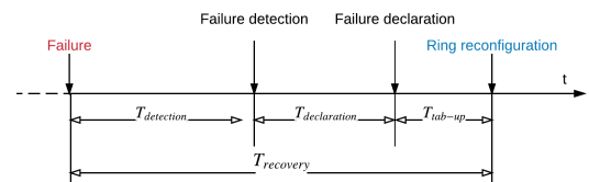
Fig. 7. Recovery time since the failure occurrence until the ring reconfiguration
