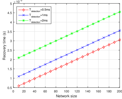
Fig. 9. The impact of T_{detection} on the Maximum Recovery Time vs the Network Size for ( M \in [10 : 10 : 200] , T_{detection} \in \{0.5, 1, 2\}ms )
