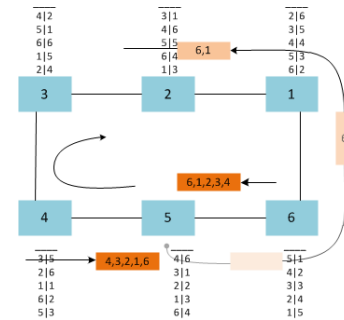
Fig. 6. The QoS-ARRP Auto-configuration Mechanism after a failure recovery
