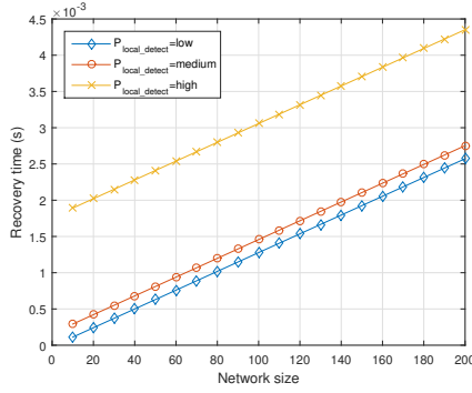
Fig. 11. The impact of P_{local\_detect} on the Maximum Recovery Time vs the Network Size for ( M \in [10 : 10 : 200] , N_{detect} = 3 , P_{local\_detect} \in \{low, medium, high\} )
