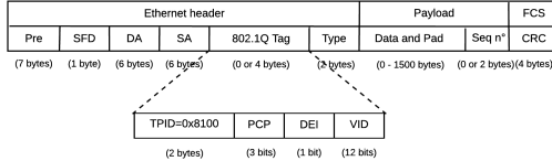
Fig. 2. QoS-ARRP frame structure
