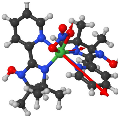
Fig. 0.3 The [\text{Ni(II)(HIM}_2\text{-py)}_2(\text{NO}_3)]^+ molecule. The thick arrows shows the direction of the axial magnetization and the thinner arrows the two other principal axes of the \mathbf{d} tensor.
