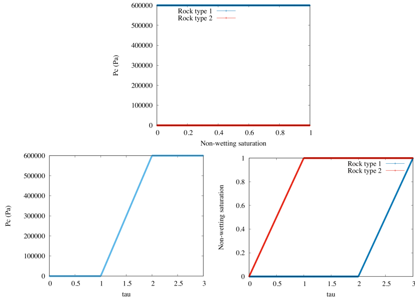
Figure 5: (Top): capillary pressure as a function of the non-wetting phase saturation for both rock types. (Bottom): capillary pressure and non-wetting phase saturations as functions of the parameter \tau \in [0, 3] .
