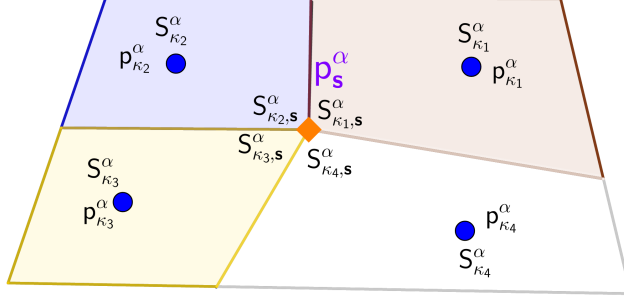
Figure 3: Discrete phase pressures and saturations in the four cells k_i, i = 1, \dots, 4 sharing the vertex \mathbf{s} .
