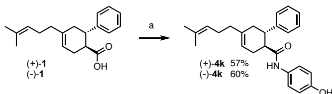
Scheme 5. Synthesis of carboxamide derivatives (+)- and (-)- 4k by peptidic coupling on (+)- and (-)-fislatic acid 1 : a) 4-Aminophenol (1.1 equiv.), HATU (1.1 equiv.), N,N -diisopropylethylamine (2 equiv.), DMF, r.t., 2 h. (+) Enantiomers correspond to 1 S ,2 S stereochemistry and (-) enantiomers to 1 R ,2 R .
