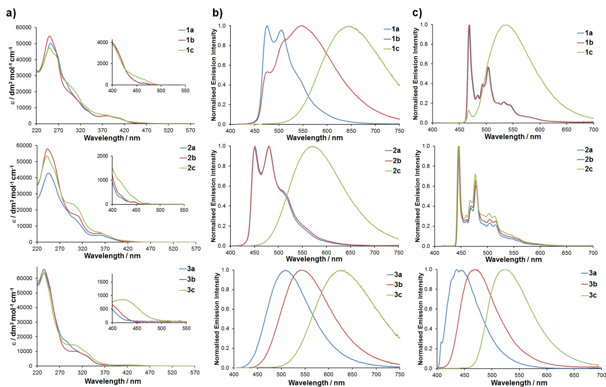
Figure 4. a) UV-Visible electronic absorption spectra recorded for MeCN solutions of 1a-3c ; b) Emission spectra for 1a-3c in aerated MeCN solution at r.t.; c) Low temperature (77 K) emission spectra recorded for 1a-3c in a glass (4:1 EtOH/MeOH).
