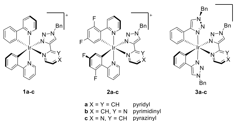
Figure 1. Structures of complexes 1a-c , 2a-c and 3a-c .
