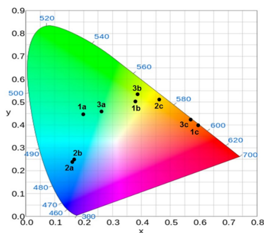
Figure 5. Commission Internationale de l'Éclairage 1931 (CIE) coordinates derived from room-temperature solution state emission spectra of complexes 1a-3c in acetonitrile.
