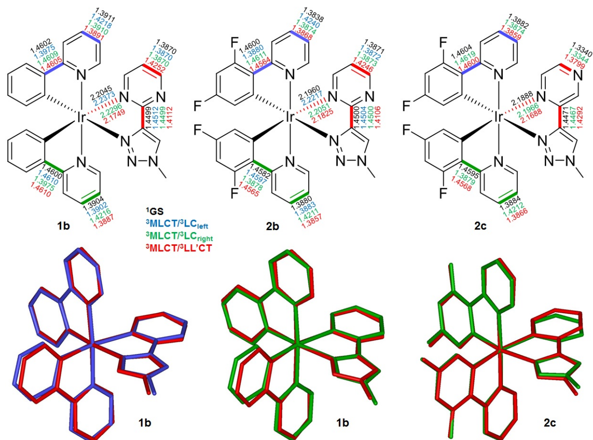
Figure 12. Top: Summary of lengths (Å) of key selected bonds (highlighted in bold) for the 1 GS (black numbers), 3 MLCT/ 3 LC left (blue numbers), 3 MLCT/ 3 LC right (green numbers) and 3 MLCT/ 3 LL'CT (red numbers) states of 1b , 2b and 2c . Bottom: overlay of equilibrium geometries for 3 MLCT/ 3 LL'CT (red), 3 MLCT/ 3 LC left (blue), 3 MLCT/ 3 LC right (green) states of 1b and 2c .
