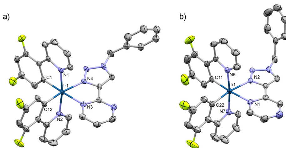
Figure 2. Molecular structures of complexes 2b (a) and 2c (b). Thermal ellipsoids are shown at 50 % probability with hydrogen atoms, co-crystallised solvent molecules and hexafluorophosphate counterions removed for clarity. Bond lengths ( \text{\AA} ) and angles ( ^\circ ) - 2b : \text{Ir}(1)\text{-N}(1) = 2.046(3) , \text{Ir}(1)\text{-C}(1) = 2.008(3) , \text{Ir}(1)\text{-N}(2) = 2.043(3) , \text{Ir}(1)\text{-C}(12) = 1.999(4) , \text{Ir}(1)\text{-N}(3) = 2.159(3) , \text{Ir}(1)\text{-N}(4) = 2.137(3) , \text{N}(1)\text{-Ir}(1)\text{-C}(1) = 80.42 , \text{N}(2)\text{-Ir}(1)\text{-C}(12) = 80.59 , \text{N}(3)\text{-Ir}(1)\text{-N}(4) = 76.14 , \text{N}(1)\text{-Ir}(1)\text{-N}(2) = 170.99 , \text{C}(1)\text{-Ir}(1)\text{-N}(3) = 176.41 , \text{N}(4)\text{-Ir}(1)\text{-C}(12) = 170.88 (CCDC 1953486). 2c : \text{Ir}(1)\text{-N}(1) = 2.159(3) , \text{Ir}(1)\text{-N}(2) = 2.125(3) , \text{Ir}(1)\text{-N}(6) = 2.055(3) , \text{Ir}(1)\text{-C}(11) = 2.006(4) , \text{Ir}(1)\text{-N}(7) = 2.046(3) , \text{Ir}(1)\text{-C}(22) = 2.004(4) , \text{N}(1)\text{-Ir}(1)\text{-N}(2) = 76.41 , \text{N}(6)\text{-Ir}(1)\text{-C}(11) = 80.27 , \text{N}(7)\text{-Ir}(1)\text{-C}(22) = 80.33 , \text{N}(1)\text{-Ir}(1)\text{-C}(11) = 174.45 , \text{N}(2)\text{-Ir}(1)\text{-C}(22) = 171.45 , \text{N}(6)\text{-Ir}(1)\text{-N}(7) = 173.25 (CCDC 1953487).
