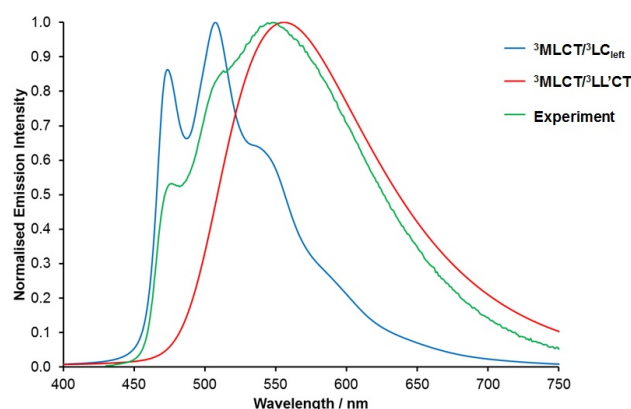
Figure 11. Comparison of calculated vibrationaly-resolved emission spectra for 1b at 300 K from the ^3\text{MLCT}/^3\text{LC}_{\text{left}} and ^3\text{MLCT}/^3\text{LL}'\text{CT} states (ethanol, SMD) with the experimentally observed emission spectrum in room temperature acetonitrile solution.
