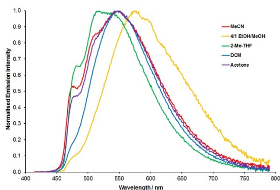
Figure 6. Normalised solvent dependent emission spectra for 1b at room temperature.
