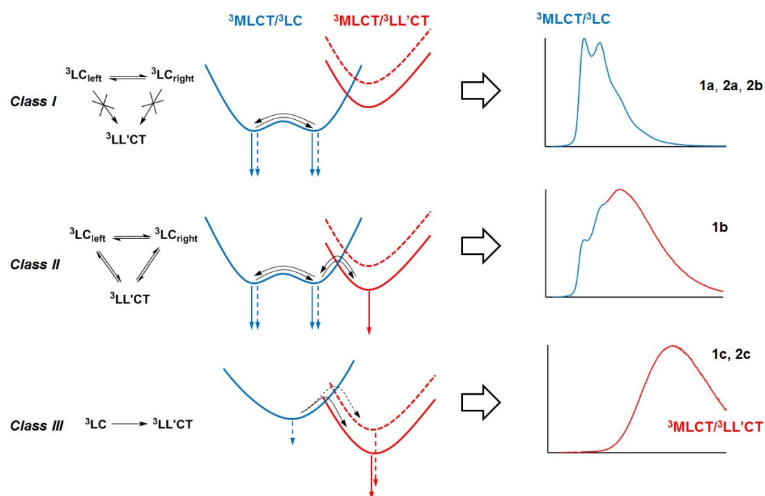
Figure 14. Qualitative potential energy surface diagram describing the excited state evolution and emission behaviour of Class I ( 1a , 2a & 2b ), Class II ( 1b ) and Class III ( 1c , 2c ) emissive [\text{Ir}(\text{C}^{\wedge}\text{N})_2(\text{N}^{\wedge}\text{N})]^+ complexes. Downward arrows represent radiative deactivation pathways. Solid lines and arrows represent processes in fluid solutions, dashed lines and arrows represent process in cryogenic glass matrices at 77 K.
