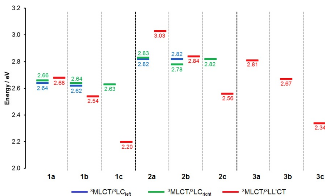
Figure 10. Calculated triplet state energies for complexes 1a-c , 2a-c and 3a-c in MeCN using SMD model. Energies are quoted relative to the optimised ground state for each complex, E GS = 0.0 eV.
