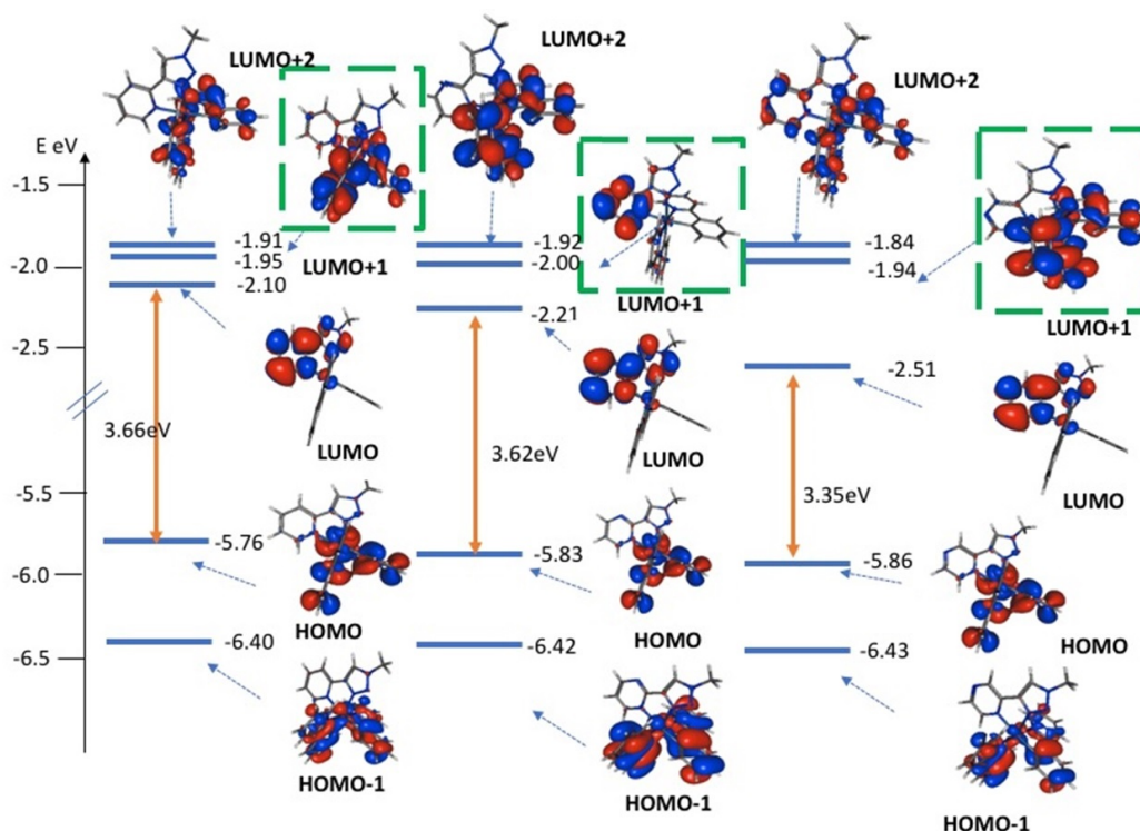
Figure 9. Molecular orbital energies and isosurface plots for HOMO-1 to LUMO+2 for complexes 1a (left), 1b (middle) and 1c (right). The green square highlights LUMO+1, whose localisation varies.
