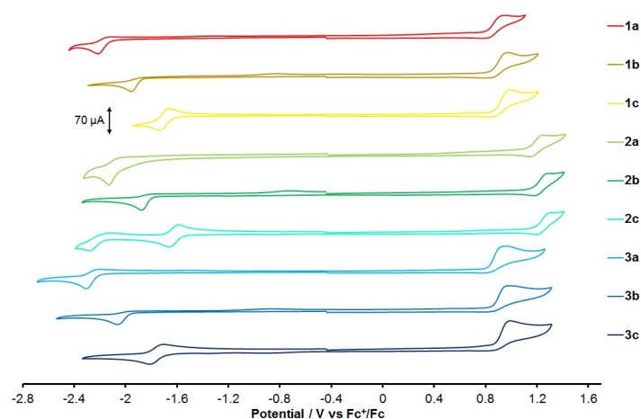
Figure 3. Cyclic voltammograms recorded for 1.6 mmoldm -3 MeCN solutions of 1a-3c at r.t. at 100 mVs -1 . Solutions contained 0.2 moldm -3 NBu 4 PF 6 as supporting electrolyte. Potentials are shown against the Fc + /Fc couple.
