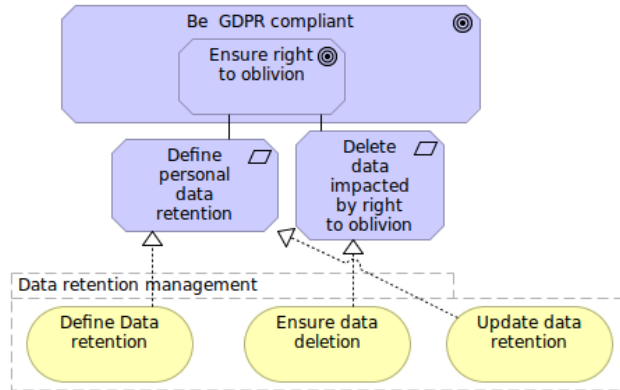
Fig. 4. Requirements and Services for Data Retention management
