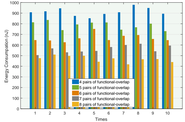
Figure 7: The energy consumption of different number of functional-overlap in concurrent service requests when PSO is executed in 10 times.
