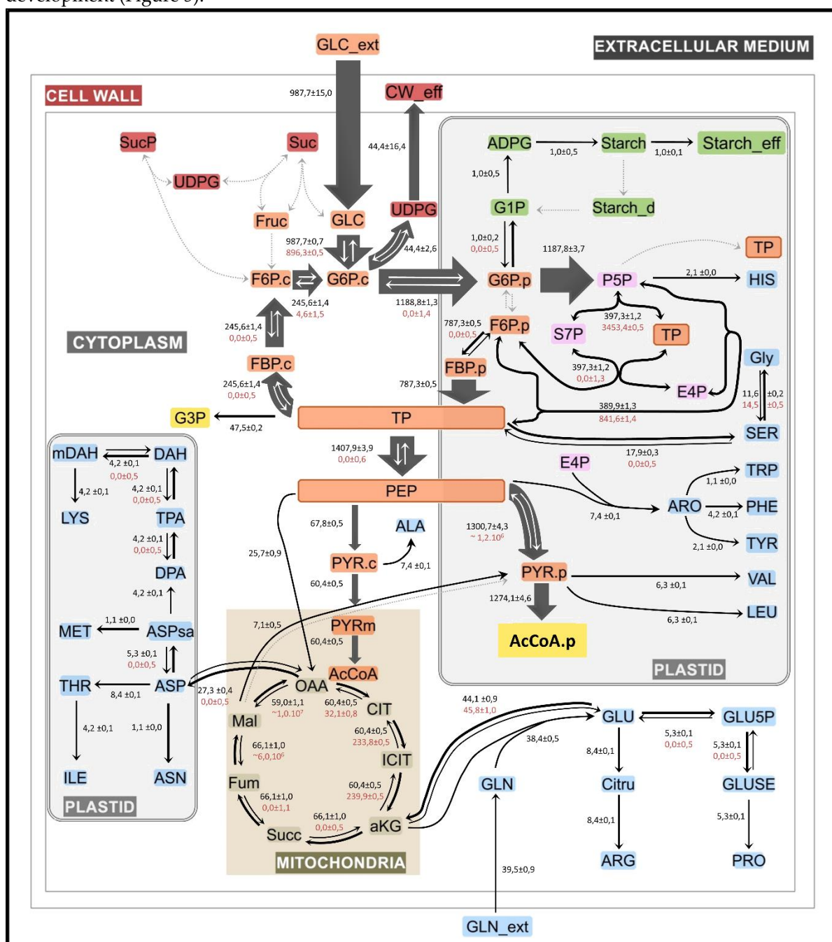
Figure 5. Metabolic network and fluxes in flaxseed embryos during maturation stage. The scheme presented is a simplified representation of the central carbon metabolism in flaxseed embryos during fatty acids synthesis and TAGs accumulation. Cytosolic and plastidial metabolites are specified by subscripts c and p, respectively, if the model distinguishes such subcellular species. All reactions, metabolites and abbreviations are available in Supplementary Table S4 and Supplementary Table S5. Values reported are the best fit obtained by INCA software using three parallel labeling experiments (53 metabolites and 6 extracellular fluxes). The average and standard deviation are calculated from four independent experiments. Fluxes are expressed in mmol/gDW/d \pm confidence interval. The set of estimated fluxes values calculated by INCA software are presented in Supplementary Table S7. The metabolic map was drawn using the Omix software [43].
