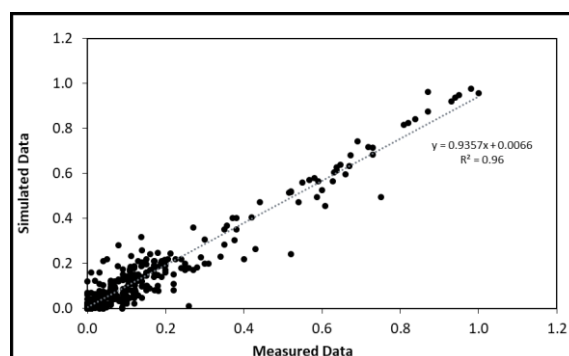
Figure 4. Comparison between predicted and measured data. The measured data correspond to the set of isotopologues of the three experimental conditions which made it possible to calculate the flux data ( n = 53 ) at 95% confidence interval and represent four biological replicates per experimental condition. These data are presented in detail in the Supplementary Table S6. The linear regression equation and R 2 value are shown.
