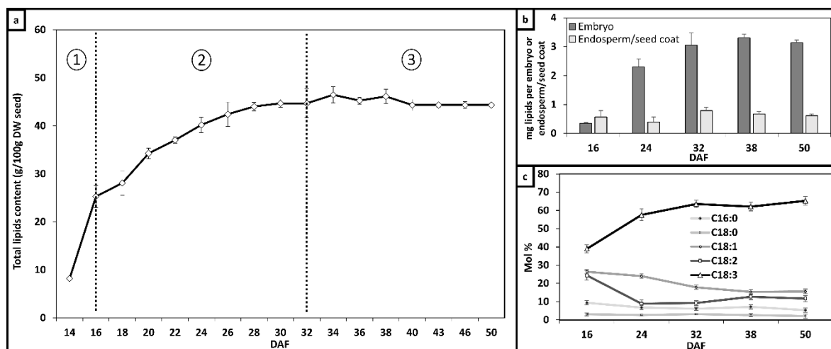
Figure 1. Synthesis of lipids and fatty acids in flaxseeds embryo and endosperm/seed coat during seed maturation. (a) Total lipids content in flaxseed expressed in g/100g DW; (b) Evolution of total lipids per tissue (mg lipids per embryo or endosperm/seed coat); (c) Relative fatty acids abundance in embryos during lipids accumulation (mol %). Data is represented as mean and variation (n = 4).
