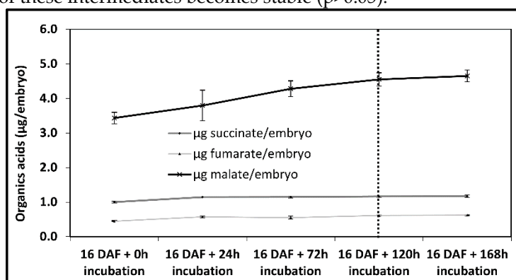
Figure 3. Concentration of organic acids ( \mu\text{g}/\text{embryo} ) during in vitro incubation. Organic acids concentrations were determined as described in Material and Method section on flaxseed embryos cultivated from 16 DAF during 24, 72, 120 and 168h in culture medium A, containing unlabeled glucose and glutamine as carbon source. For each kinetic point, four independent experiments were made.
