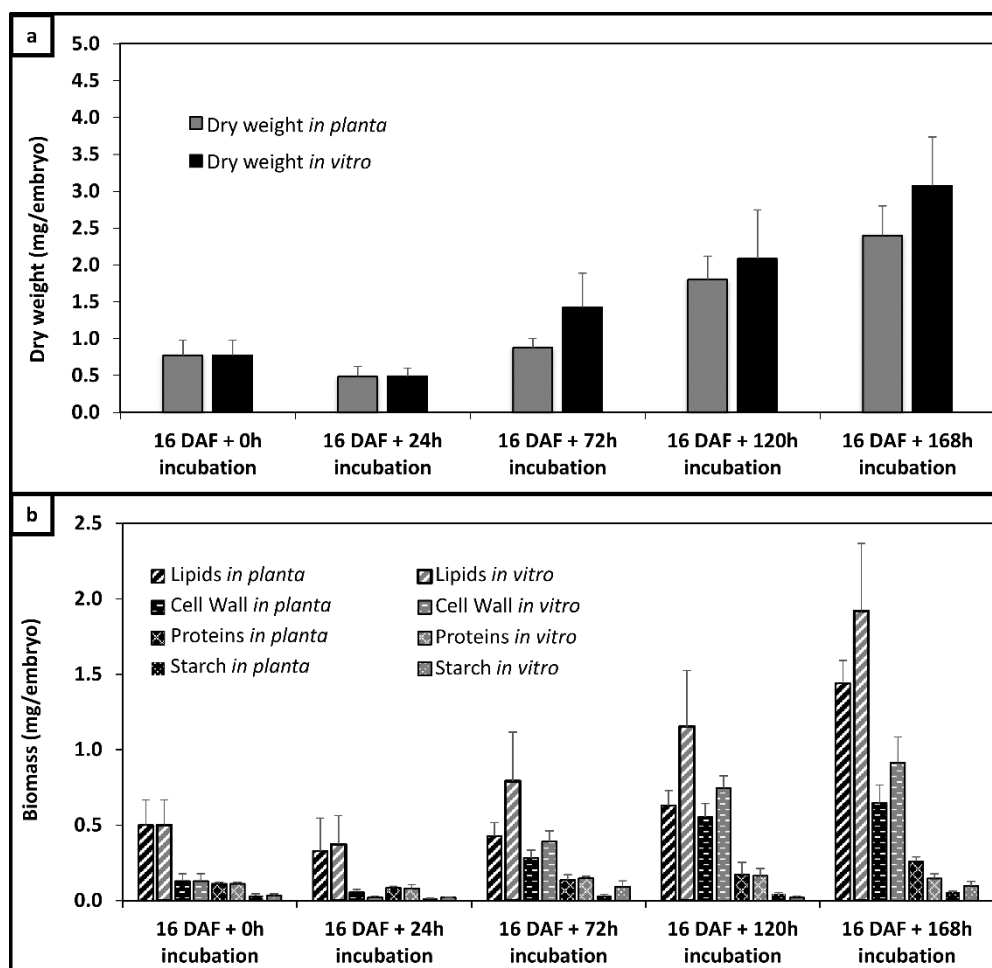
Figure 2. Weight and biomass composition between embryos cultured in vitro and its corresponding state in planta . (a) Dry weight between in planta vs in vitro expressed in mg/embryo; (b) Biomass accumulation between in vitro and in planta expressed in mg/embryo. Dry weight and biomass composition (lipids, proteins, cell wall and starch) content were determined as described in Material and Method section on flaxseed embryos cultivated from 16 DAF during 24, 72, 120 and 168h in culture medium A, containing unlabeled glucose and glutamine as carbon source. For each kinetic point, four independent experiments were made.
