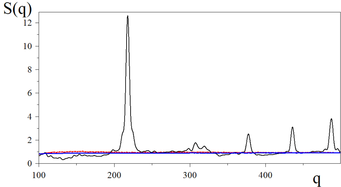
Figure 6. Structure factor (black curve) of the ensemble of spheres shown on Fig.5, built using the LL algorithm up to level 3. The restricted Bragg peaks are due to the limited regular packing sets inherent to the LL algorithm. The variable q is counted in units determined by the choice of the unit length (the edge of the cube). For comparison, the dotted red curve is the structure factor of an Apollonian packing, as discussed in [17], and the blue curve quite close to value 1 is for packing obtained using the Manna's algorithm, as discussed in [13]. In these three examples, the systems were made of about 800 000 spheres, and angle-averaging was performed with 25 000 random Euler angles. No Bragg peak is seen either in the Apollonian packing or in the Manna packing structure factor.
