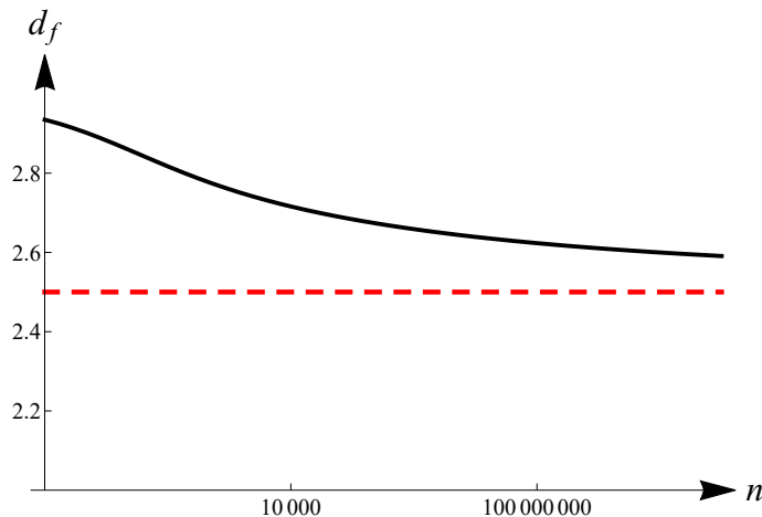
Figure 4. Solution (black curve) in d_f of the equation (33) versus the variable n . The red dashed line is the special value d_f = 5/2 . The asymptotic solution for n \rightarrow \infty is d_f \simeq 5/(2 - \log 6/\log n) \rightarrow 5/2 . This figure shows that, for given value of d_f , the inequation (32) has solution in n only if d_f > 5/2 .
