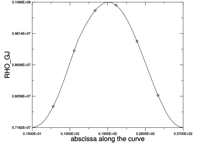
Fig. 6. Values of the Goldreich-Julian density on the NS surface at the foot of the last open magnetic field lines for a dipole magnetic field of inclination i = 40 deg.
