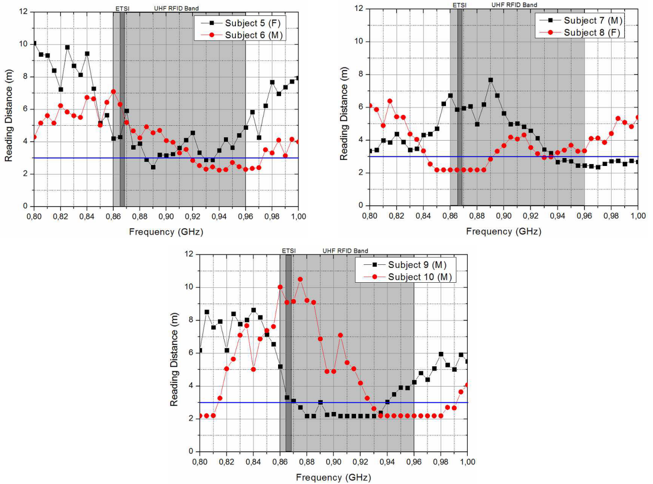
Figure 25. Measured readings distances on several people.
