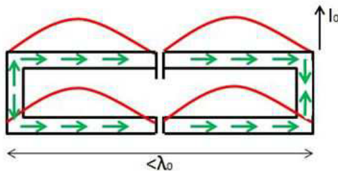
Figure 15. Current distribution on a folded dipole with a length of 2\lambda_0 .
