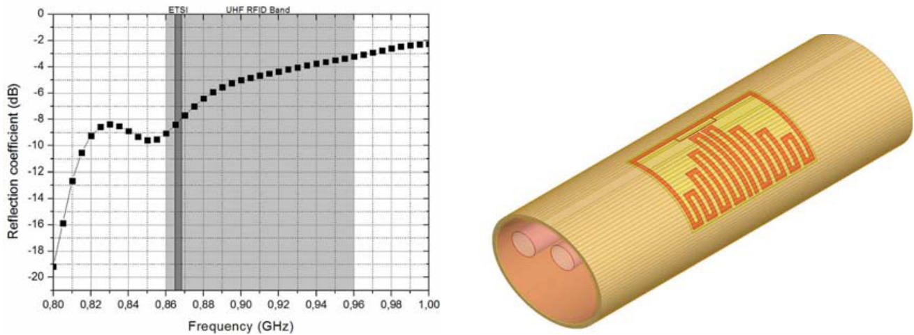
Figure 22. Tag on the forearm and its reflection coefficient.
