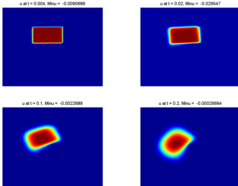
Figure 3: Test 4: The approximate density for simulation times t_1 = 0.004 , t_2 = 0.02s , t_3 = 0.1 and t_4 = 0.2 using a centered scheme without correction.
