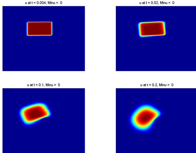
Figure 4: Test 4: The approximate density for simulation times t_1 = 0.004 , t_2 = 0.02s , t_3 = 0.1 and t_2 = 0.2 . using the positive scheme (3.1)-(3.2).
