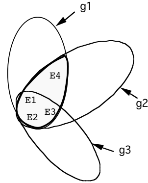
Fig. 3. The equivalence needed to allow the study of conditions on the local bias. The effect of the local bias (forgetting of some element of the S-set or G-set) is the same as the effect of additional instances made available to an order independent algorithm such as the CE algorithm.
