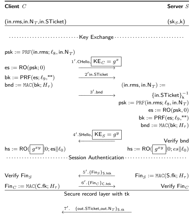
Fig. 2. Our modelling of the TLS 1.3 handshake- session resumption, both presared key-only and presared key with Diffie Hellman key exchange. In the boxes we have the protocol elements specific to the pre-shared key with Diffie-Hellman key exchange mode. We have prefixed the N_T , rms, STicket used at the beginning of the session with in, and those created at the end of a session by out. This emphasises they are different variables.
