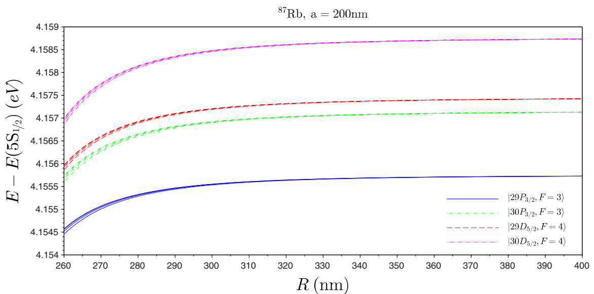
FIG. 18. Lamb shift of an ^{87}\text{Rb} atom in the states |nP_{3/2} F = 3, M_F = -F \dots F\rangle and |nD_{5/2} F = 4, M_F = -F \dots F\rangle , for n = 29, 30 near an optical nanofiber. We represent the energy difference, E - E(5S_{1/2}) , of the states of interest with respect to |5S_{1/2}\rangle as a function of the distance, R , from the fiber. The radius of the nanofiber is a = 200 nm. Energies are given in eV.
