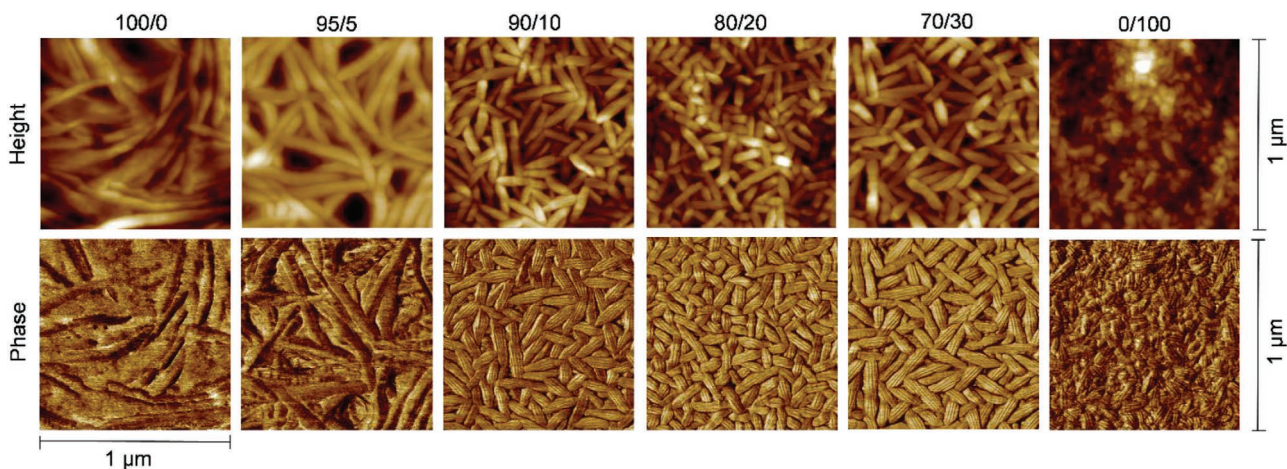
Figure 5. AFM images of height and phase of fluorinated polymer blend films at different terpolymer/copolymer ratios (100/0, 95/5, 90/10, 80/20, 70/30, 0/100) (tapping mode, 1 µm × 1 µm scan area).
