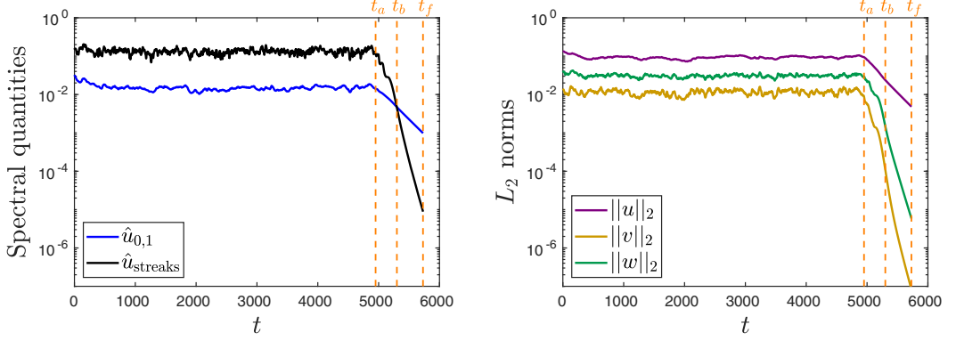
FIG. 8. Time evolution of spectral quantities \hat{u}_{0,1} and \hat{u}_{\text{streaks}} (left) and of L_2 norms \|u\|_2 , \|v\|_2 , and \|w\|_2 (right) for a decay event at \text{Re} = 830 . Times t_a , t_b , and t_f refer to slices shown on Fig. 5. The band starts to decay at t_a , \hat{u}_{0,1} = \hat{u}_{\text{streaks}} at t_b , and the relaminarization is considered as complete at t_f .
