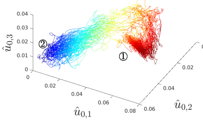
FIG. 13. Evolution of spectral quantities during ten splittings at \text{Re} = 1200 , in a domain of length L_z = 50 . Each curve represents one simulation, and is colored by \hat{u}_{0,1} to illustrate the transition between a one-band (1) and a two-band state (2).
