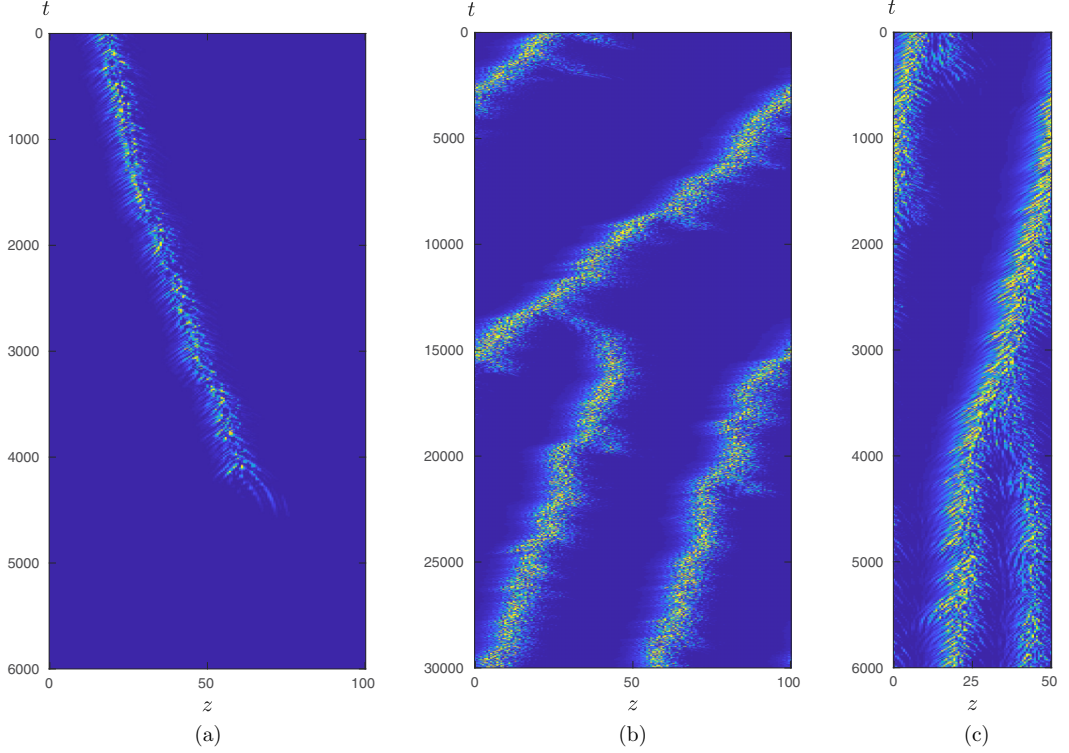
FIG. 2. Space-time diagrams of turbulent bands in a frame moving at the bulk velocity, U_{\text{bulk}} , with (a) \text{Re} = 830 , L_z = 100 , (b) \text{Re} = 1100 , L_z = 100 , (c) \text{Re} = 1200 , L_z = 50 . Colors show the perturbation energy E = \frac{1}{2}(u^2 + v^2 + w^2) as a function of z and t , sampled in the y = -0.8 plane at an arbitrary value of x (yellow: E = 0.1 ; blue: E = 0 ). Average band propagation velocities, relative to U_{\text{bulk}} , and the degree of fluctuations can be discerned from diagrams. Case (a) is an example of a band moving downstream relative to U_{\text{bulk}} , which occurs for \text{Re} \lesssim 1000 , and then decaying. In case (b), a single band in a domain with L_z = 100 splits into two bands, resulting in a pair of bands separated in z by distance 50 = L_z/2 . The change in velocity resulting from a decrease in interaction distance is evident. Note, however, that the time range covered in the plot is large, which visually accentuates the effect. Case (c) shows band splitting in a domain of size L_z = 50 . The resulting bands are closely spaced and interact strongly.
