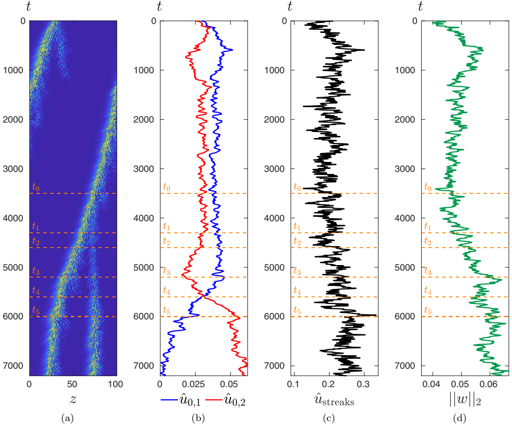
FIG. 11. Evolution of a band while it splits at \text{Re} = 1200 . (a) Spatiotemporal diagram of the band. Colors show the turbulent perturbation energy E between 0 (blue) and 0.1 (yellow). (b)–(d) Time evolution of spectral quantities \hat{u}_{0,1} and \hat{u}_{0,2} (b), \hat{u}_{\text{streaks}} (c), and the L_2 -norm \|w\|_2 (d).
