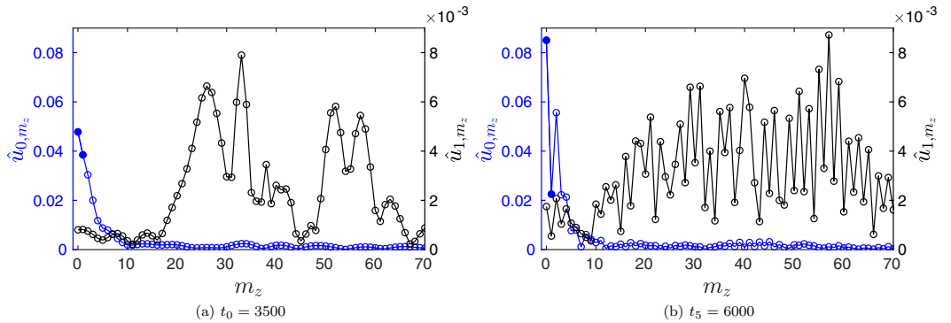
FIG. 12. Illustrative Fourier spectra \hat{u}_{0,m_z} and \hat{u}_{1,m_z} (a) before and (b) after band splitting at \text{Re} = 1200 . The black symbols \hat{u}_{1,m_z} correspond to streaks while the blue symbols \hat{u}_{0,m_z} at low m_z correspond to large-scale structures. Filled symbols indicate \hat{u}_{0,1} and \hat{u}_{0,2} .
