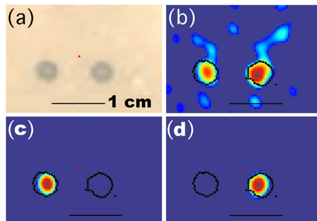
FIG. 4. (Color online) (a) Photography of the two dyed microbubbles dot. (b) Acoustic field collected by the hydrophone. [(c) and (d)] Separation of the two microbubbles dots. Acoustic field after geometric projection and selection.
