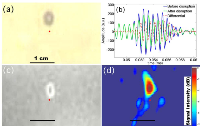
FIG. 2. (Color online) (a) Photography of the dyed microbubbles dot. (b) Echo of a weak interrogation pulse on the gelatin surface on a single element. (c) Photography of the color change on the thermosensitive paper. (d) Acoustic field collected by the hydrophone. The red dot is the geometric focal point, the black line is 10 mm long and the colorbar scale is dB relative to the maximum.
