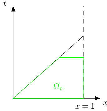
Figure 18: The domain \Omega_t
