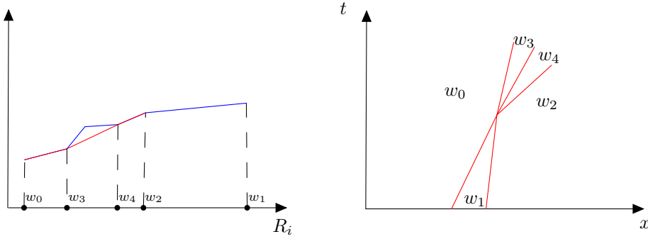
Figure 14: Not all jumps have the same sign
