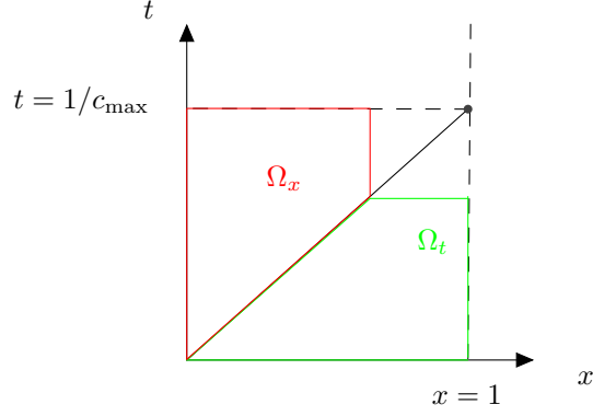
Figure 19: The domain \Omega_x
