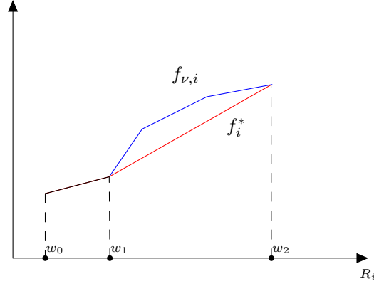
Figure 10: The case R_i^l < R_i^r
