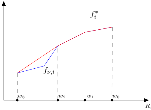
Figure 11: The case R_i^l > R_i^r
