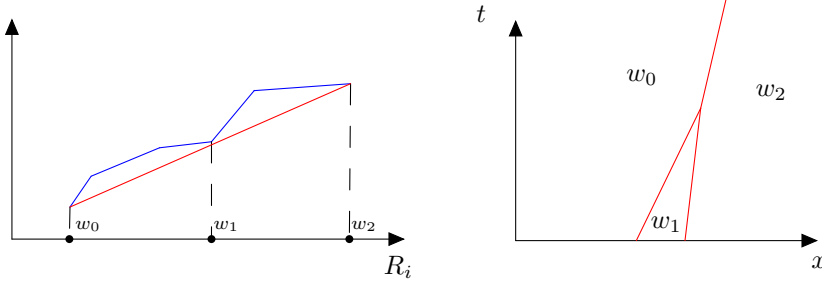
Figure 13: All jumps have the same sign
