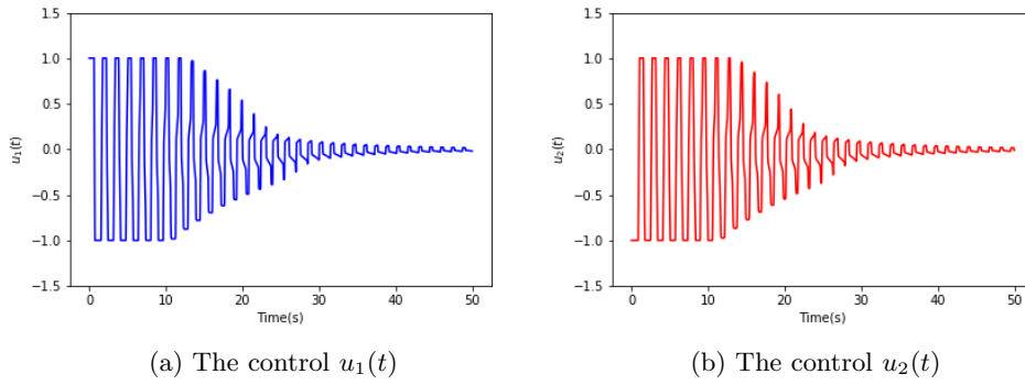
Figure 7: The case R_0(x) = (15, -15)
