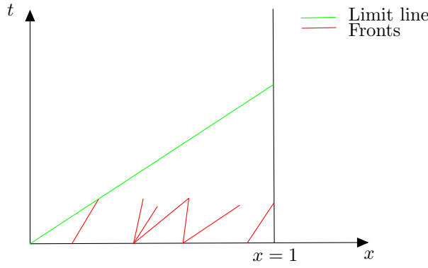
Figure 12: The local in time solution
