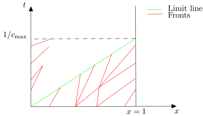
Figure 16: The local solution above the limit line
