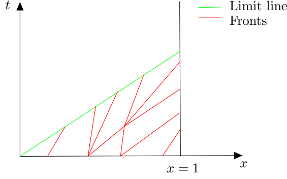
Figure 15: The solution under the limit line
