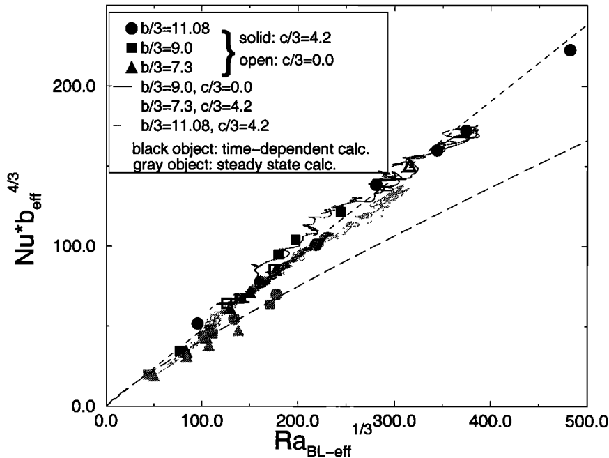
Figure 12. Nu \times \frac{1}{2} \left( b - 2.6 \frac{c}{Nu} \right)^{4/3} plotted versus Ra_{\text{BL-eff}}^{1/3} for a non-Newtonian rheology, with time-dependent and steady state calculations. A linear regression of the form y = a_1 x for the turbulent regime yields a_1 = 0.48 (short-dashed line). Nonlinear curve fitting of the form y = a_2 x^{a_3} for the stationary regime yields a_2 = 0.75 and a_3 = 0.87 (long-dashed line). Black symbols are pictured for time-dependent calculations and gray symbols for steady state calculations. Open symbols represent simulations done with no pressure dependence of the viscosity. Solid symbols show simulations done with a temperature dependence of the viscosity of b/3 = 11.08 , squares are calculated with b/3 = 9.0 , and triangles are calculated with b/3 = 7.3 . Solid, heavily shaded, and lightly shaded lines represent simulations for which Ra_0 has been increased slowly, with a temperature dependence of the viscosity of b/3 = 11.08 , b/3 = 9.0 , and b/3 = 7.3 , respectively.
