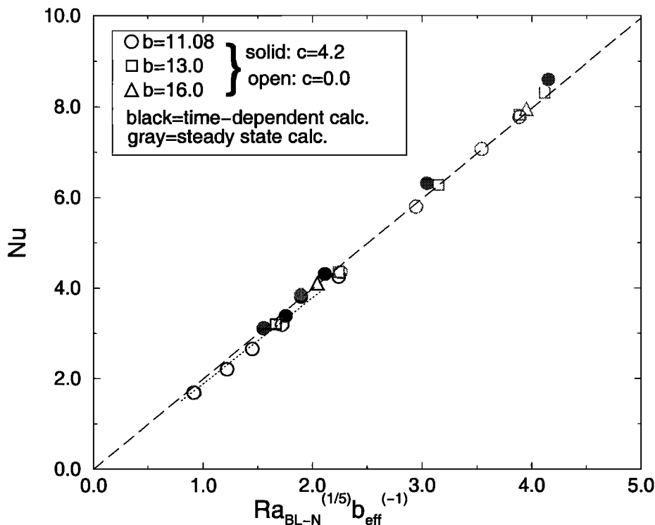
Figure 10. Nusselt number plotted versus Ra_{BL-N}^{1/5} b_{eff}^{-1} , for stationary flows resulting from either time-dependent or steady state calculations. Long dashed line is Fowler [1985]'s prediction and dotted line represents Moresi and Solomatov's [1995] results (symbols as in Figure 5).
