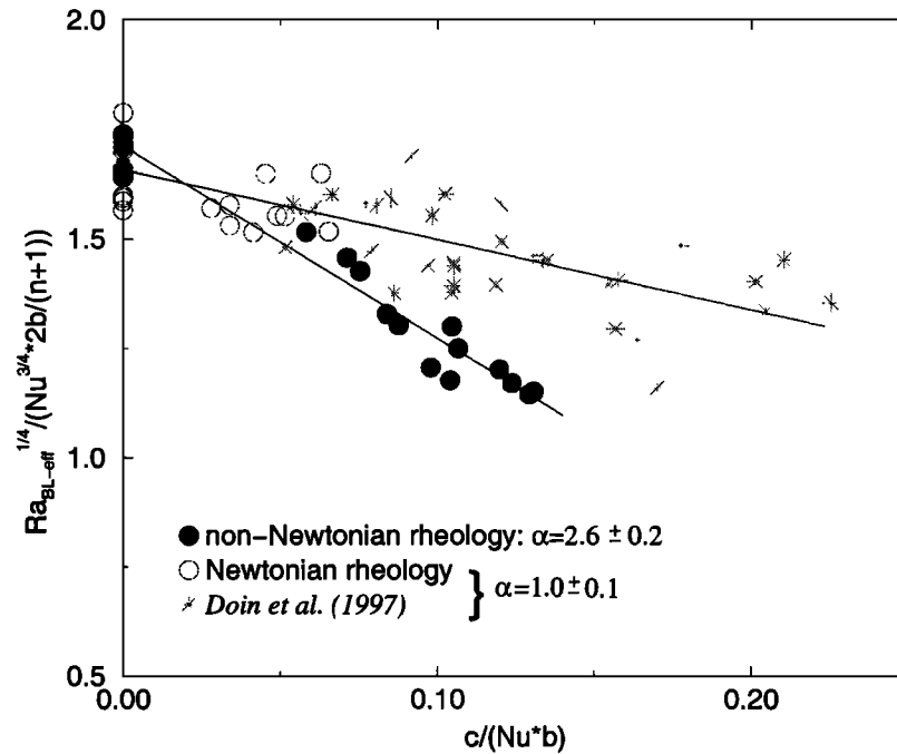
Figure 7. Linear regressions performed to compute \alpha in Nu = \beta_1 Ra_{BL-eff}^{1/3} \{ [2/(n+1)] (b - \alpha c / Nu) \}^{-4/3} for turbulent flows. The rheology is Newtonian for open circles (this study) or asterisks [Doin et al. , 1997], and non-Newtonian for solid circles.
