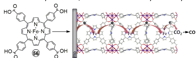
Figure 16. Fe-porphyrin based metal-organic frameworks (MOFs) for the modification of cathodes in the heterogeneous electrocatalytic \text{CO}_2 reduction. Adapted with permission from Ref. 87.
