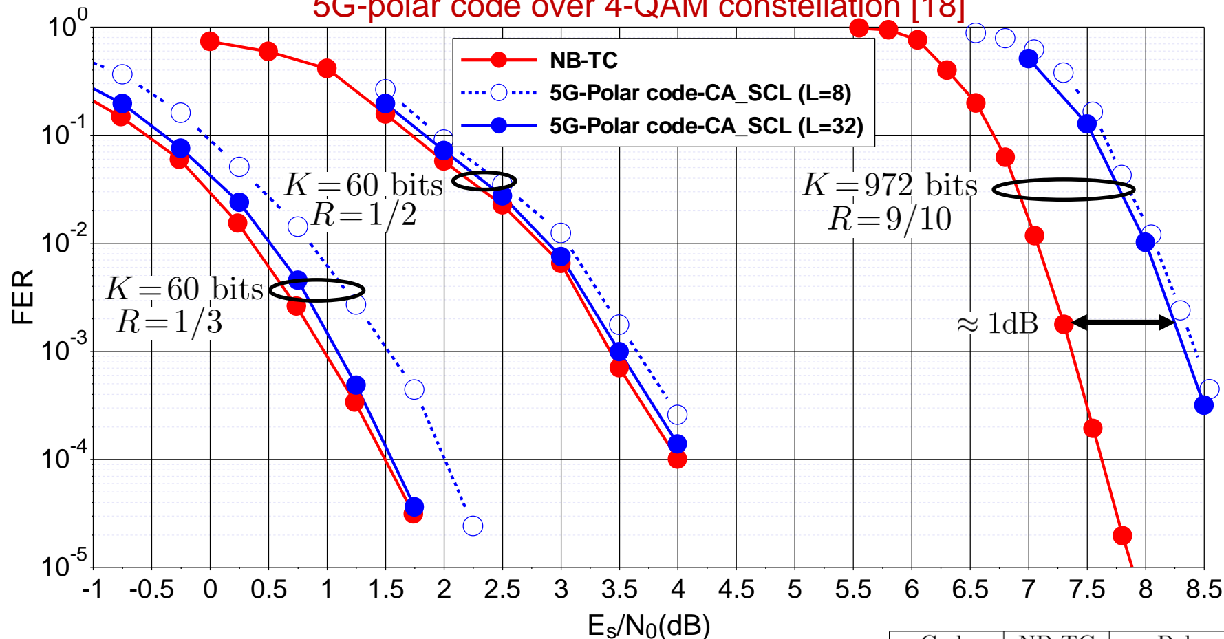
Frame error rate performance comparison of NB-TCs and 5G-polar code over 4-QAM constellation [18]
