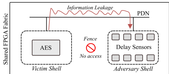
Fig. 2: Threat Model – A FPGA fabric is divided into multiple user shells. Logical isolation between each tenant is provided by fences but a side-channel attack can be conducted thanks to the information leakage that propagates throughout the PDN.
