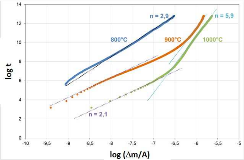
Figure 7: Analysis of the oxidation kinetics of the SPSed specimens (produced from Ti_3AlC_2 powder densified at 1315°C/75MPa/2min) after oxidation in the temperature range 800-1000°C during 100h in synthetic air.
