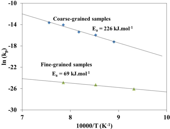
Figure 8: Arrhenius plot of the parabolic rate constant as a function of the inverse temperature for the coarse-grained (diamond) and fine-grained (triangle) specimens.
