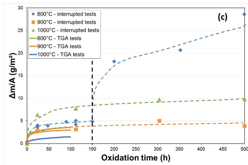
Figure 6: \Delta m/A plotted as a function of oxidation time, in synthetic air, in the temperature range 800-1000°C. (a) for SPSed samples produced from \text{Ti}_3\text{AlC}_2 powder densified at 1315°C/75MPa/2min, (b) for HIPed samples produced at 1450°C/2h and 50MPa/1h, (c) for SPSed samples with a comparison between ambient air and TGA oxidation tests.
