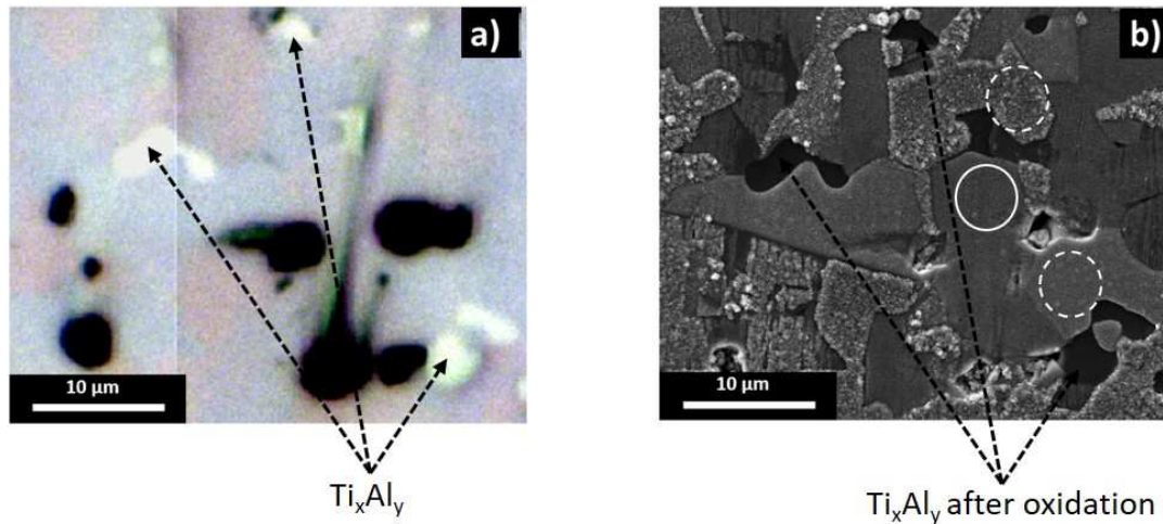
Figure 14: (a) white light OM observation of the SPSed sample produced from \text{Ti}_3\text{AlC}_2 powder densified at 1315^\circ\text{C}/75\text{MPa}/2\text{min} . Black areas are either alumina or pores whereas light grey and white areas are respectively \text{Ti}_3\text{AlC}_2 and \text{Ti}_x\text{Al}_y phases. (b) a SEM observation of the same region after 60 min of oxidation at 800^\circ\text{C} .
