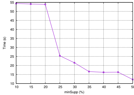
Fig. 2. Evolution of the computation time for discovering seasonal gradual patterns vs the variation of the minSupp value.
