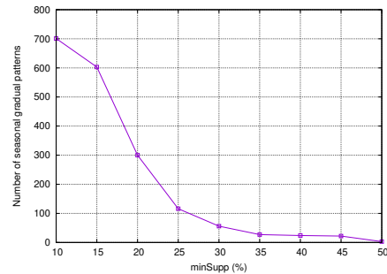
Fig. 1. Number of seasonal gradual patterns with minSupp variation.
